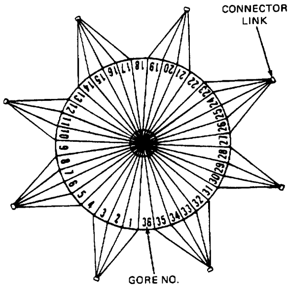
Suspension Line Arrangement Numbering
